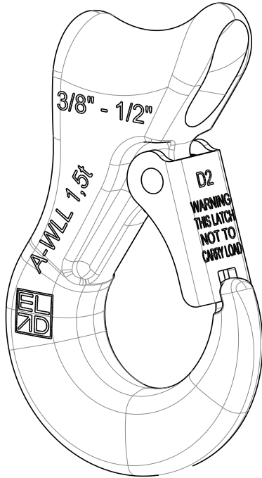
Item 8062 Sliding choker hook
